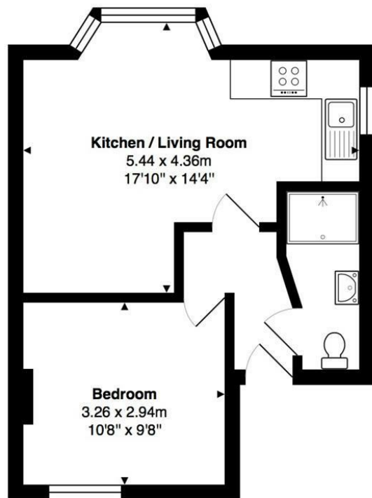
Second Floor Area: 34.4 m 2 ... 370 ft 2 Heat-Loss Perimeter: 3.6m ... 12ft
